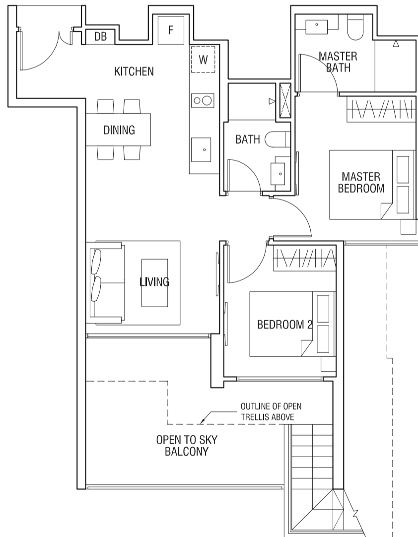
Lower Storey
