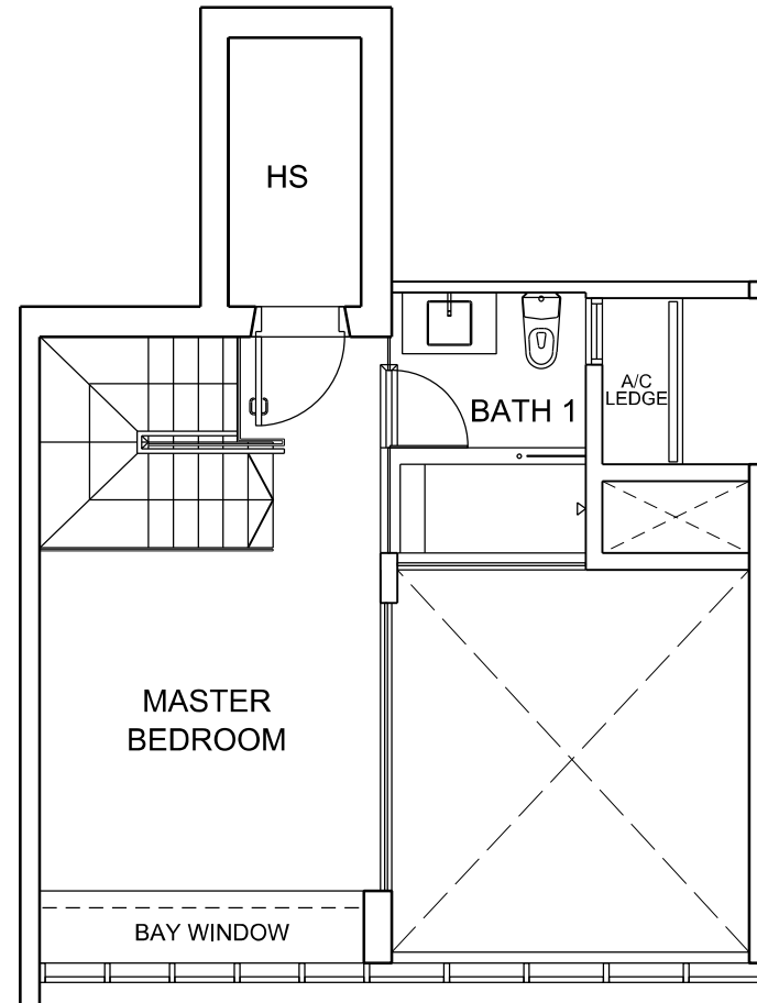
UPPER STOREY
