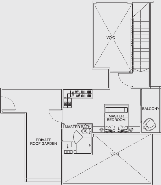
ATTIC
