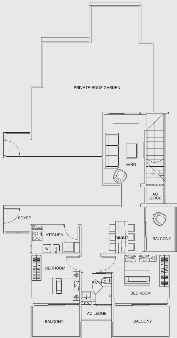
5th STOREY
