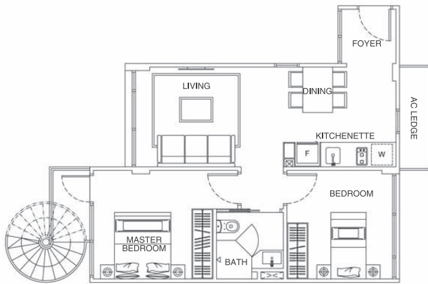
5th STOREY
