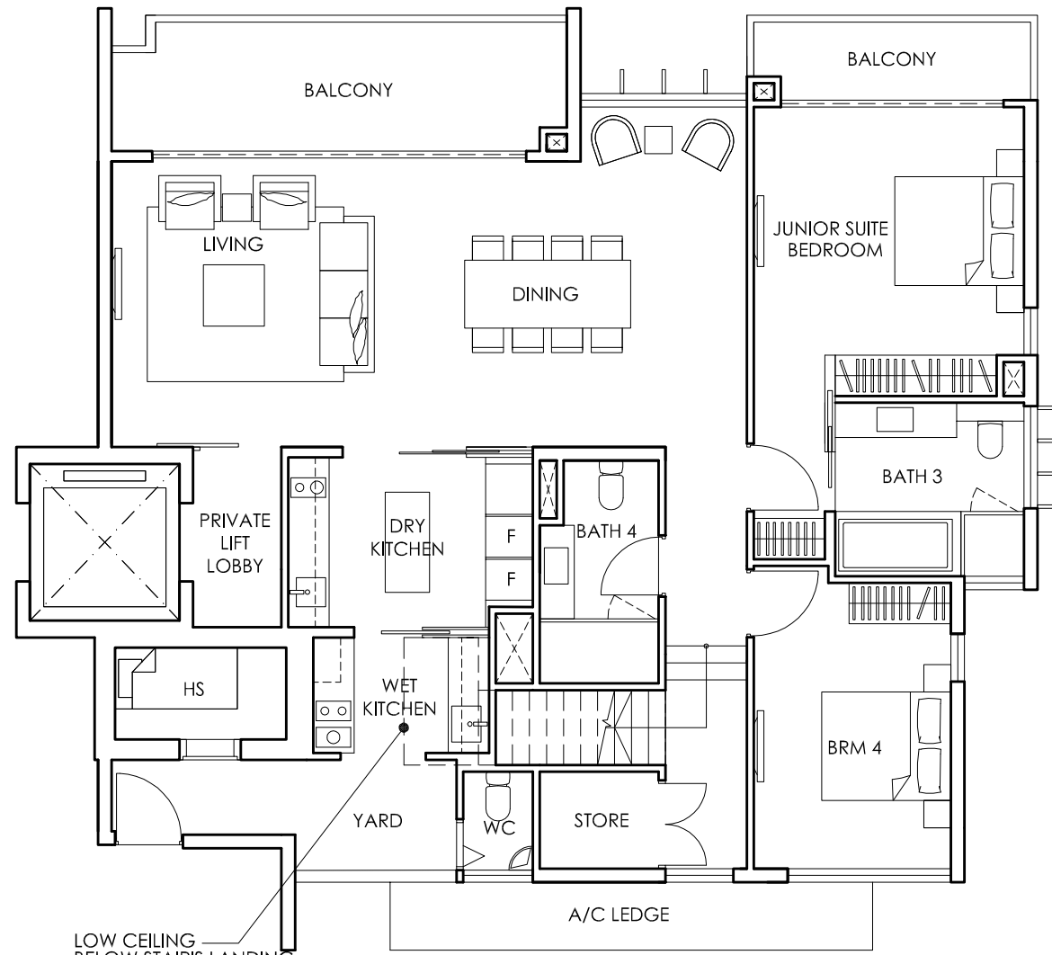
LOWER LEVEL
