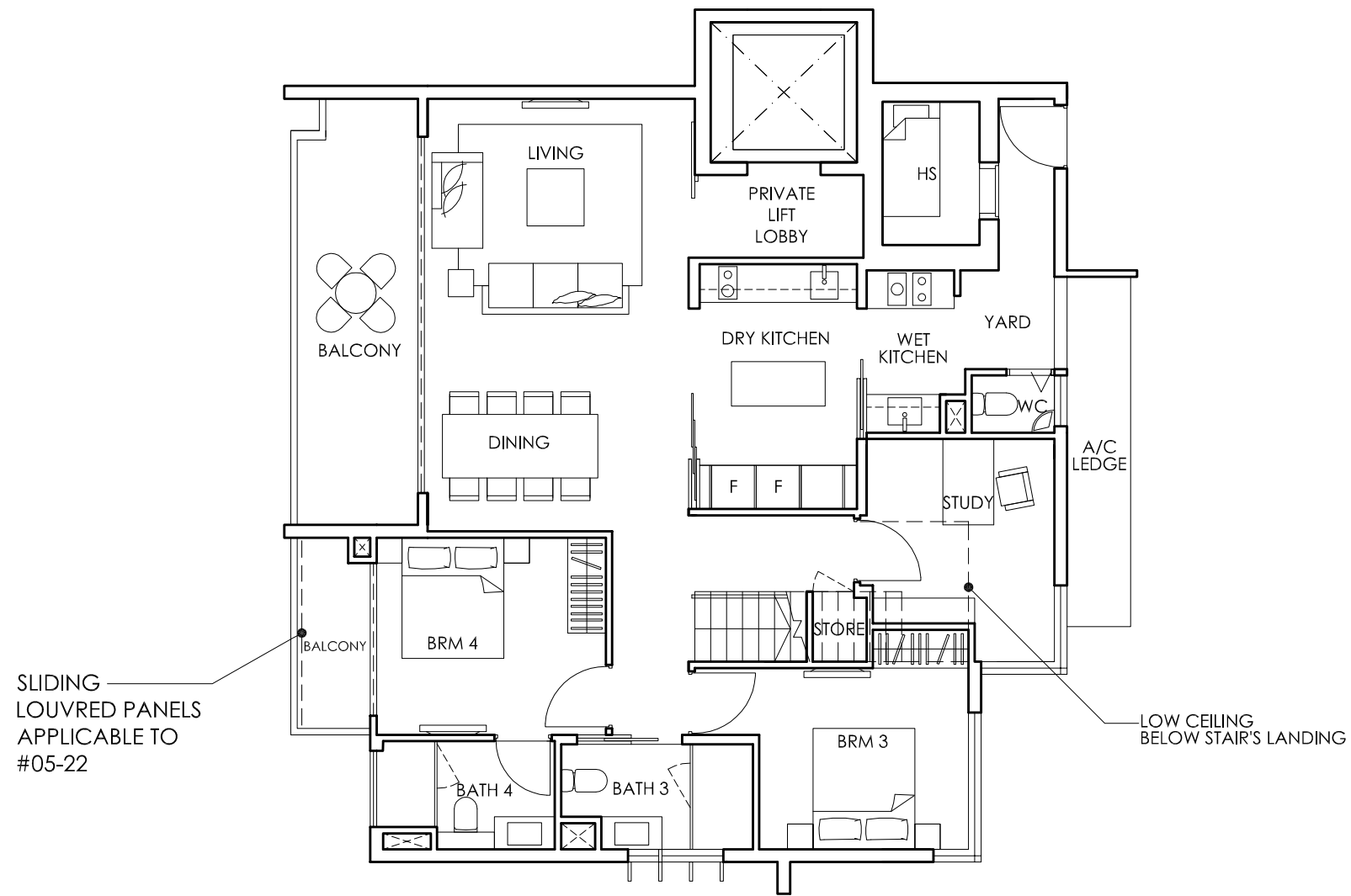
LOWER LEVEL
