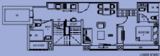
LOWER STOREY
