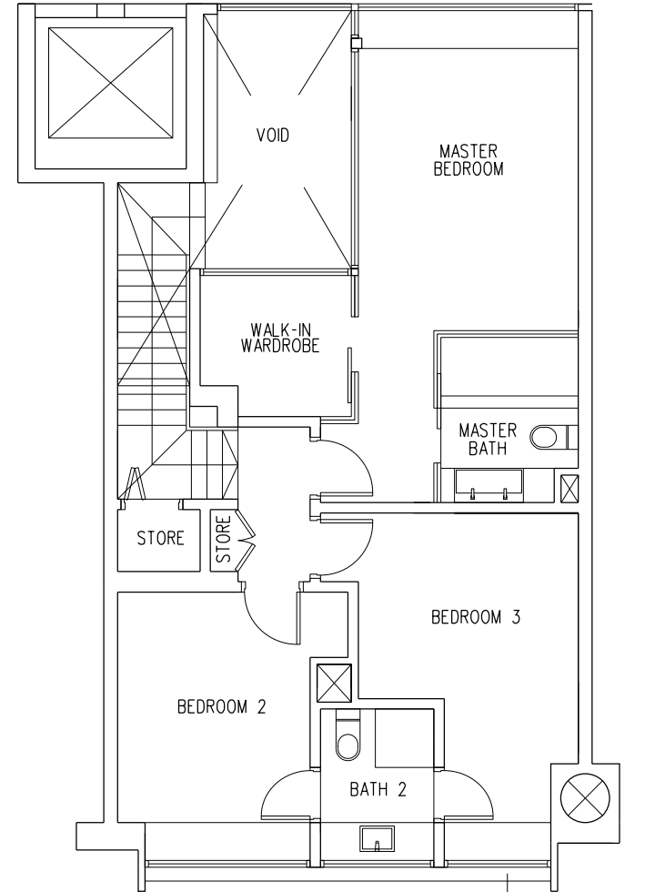
UPPER STOREY
