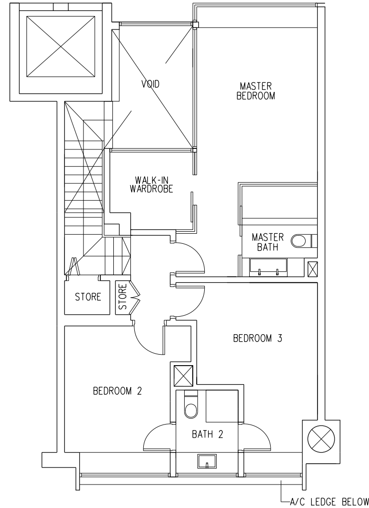
UPPER STOREY
