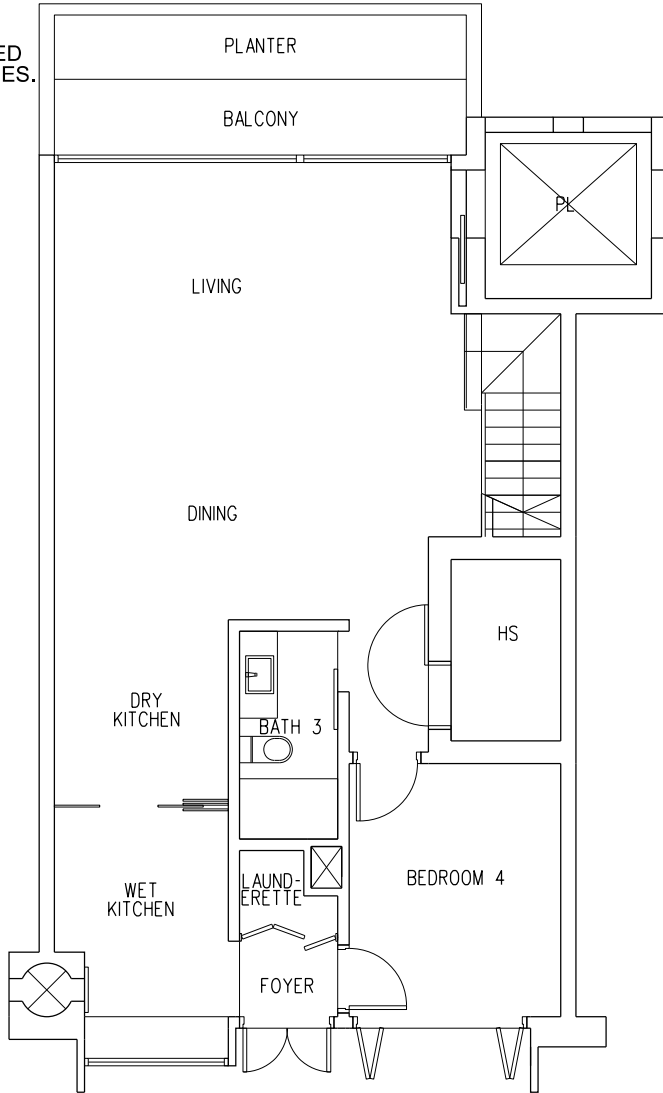
LOWER STOREY
