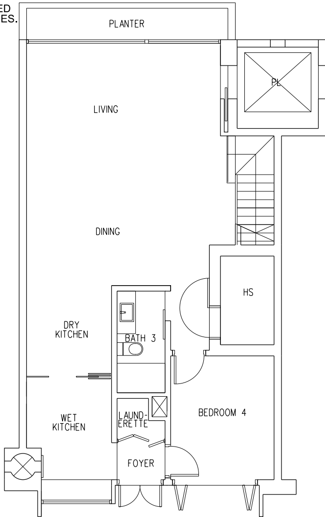
LOWER STOREY
