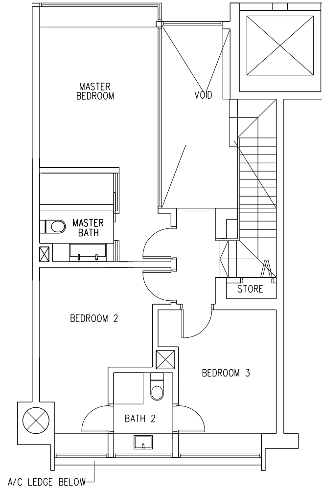
UPPER STOREY
