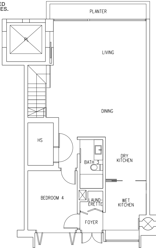
LOWER STOREY
