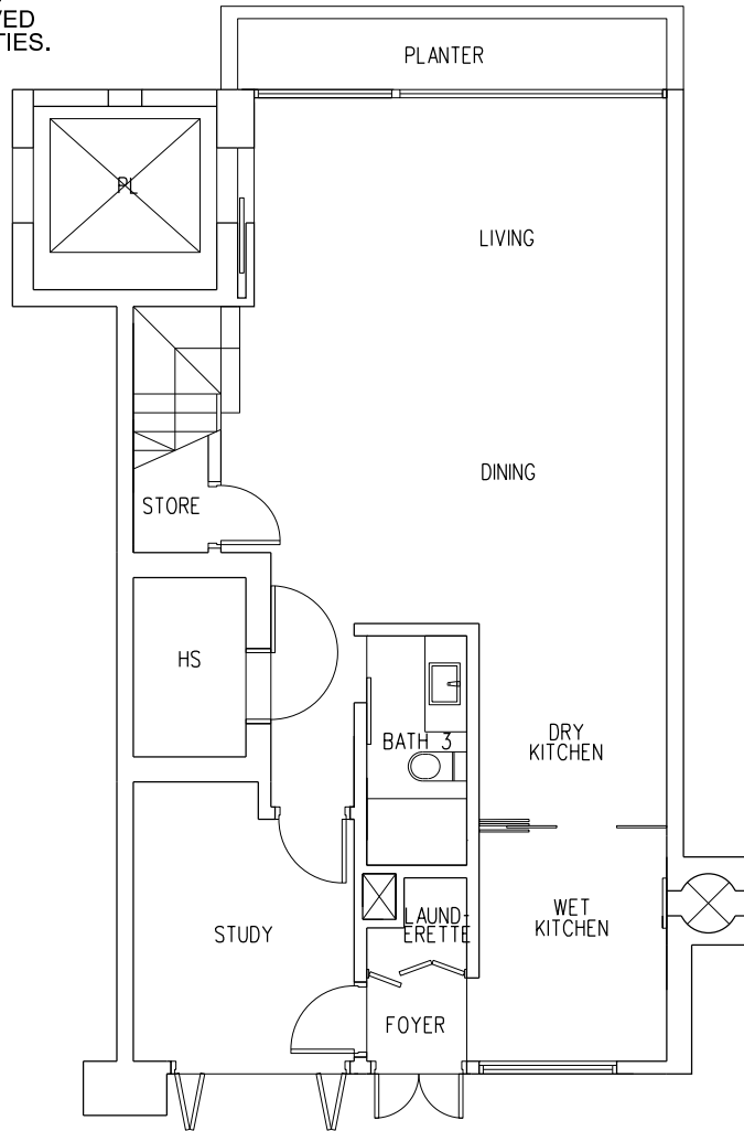
LOWER STOREY
