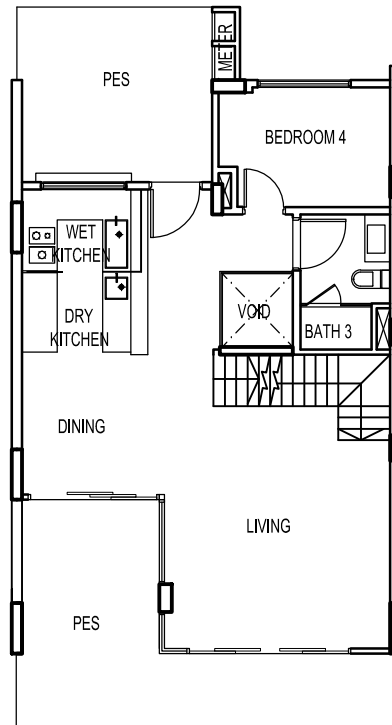
1ST STOREY PLAN
