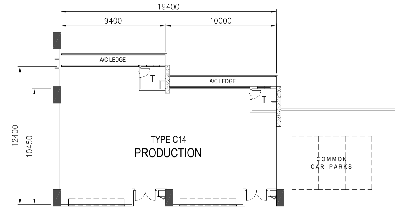
TYPE C14 - 5TH to 8TH STOREY PLAN
