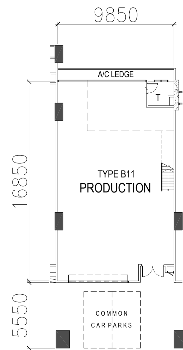
TYPE B11 - 2ND to 3RD STOREY PLAN
