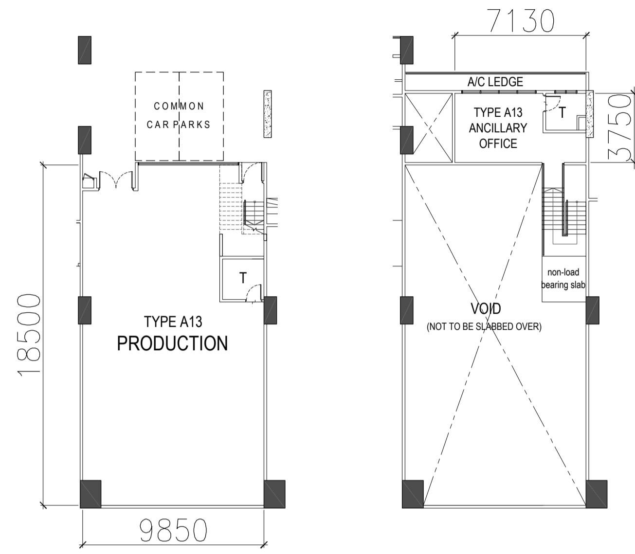
TYPE A13 - 1ST STOREY PLAN
