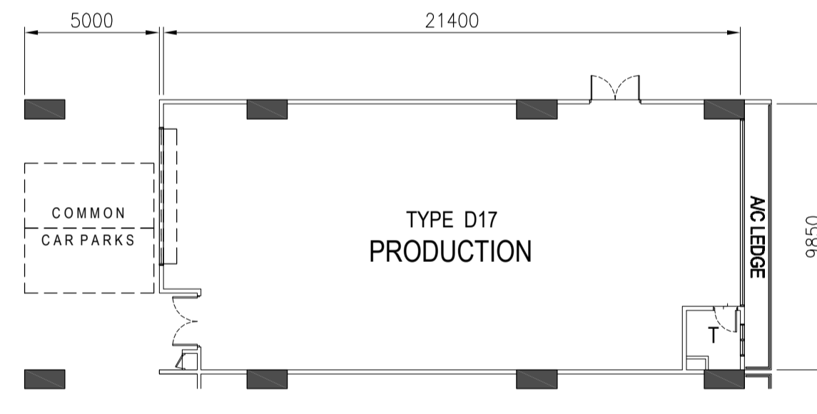
TYPE D17 - 9TH STOREY PLAN
