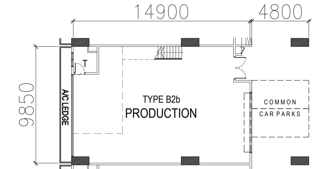
TYPE B2b- 2ND to 3RD STOREY PLAN
