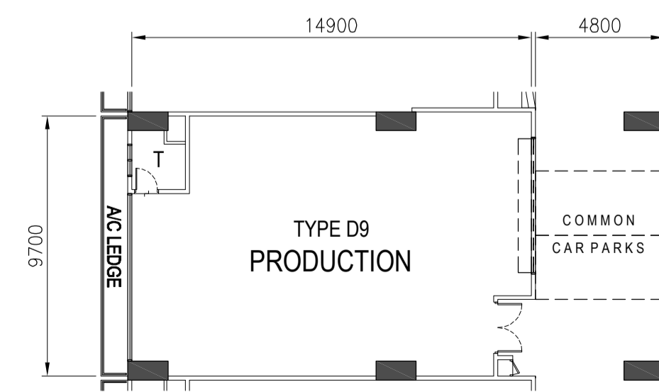
TYPE D9 - 9TH STOREY PLAN
