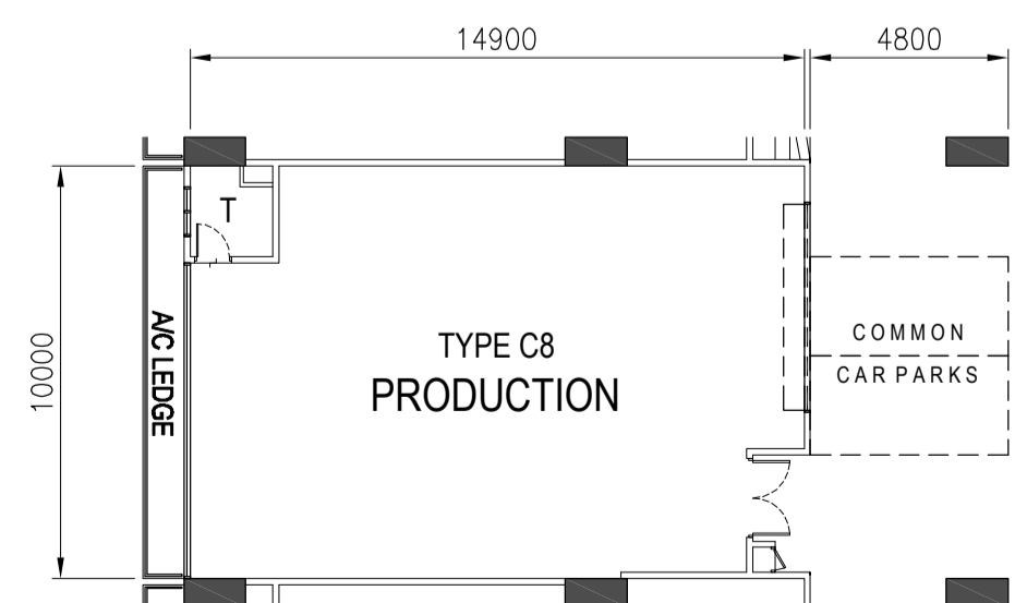
TYPE C8 - 5TH to 8TH STOREY PLAN
