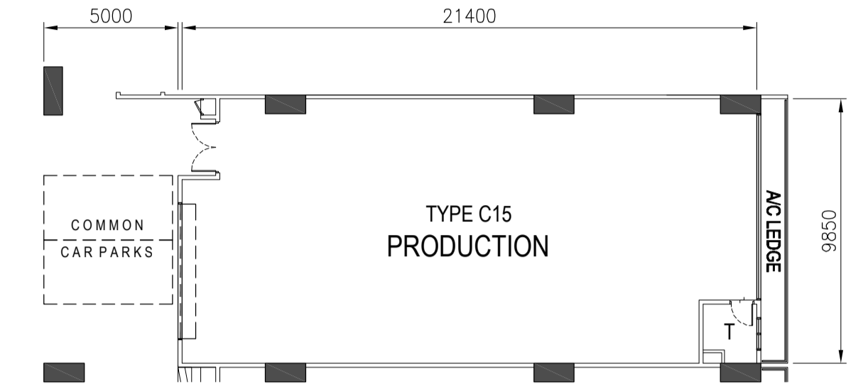
TYPE C15 - 5TH to 8TH STOREY PLAN
