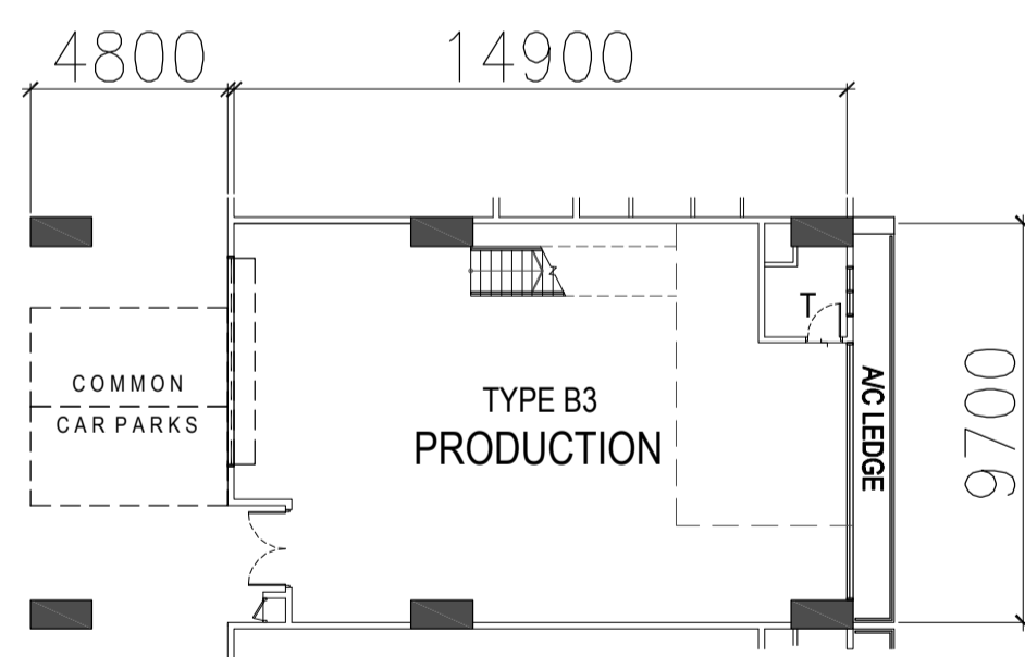
TYPE B3- 2ND to 3RD STOREY PLAN
