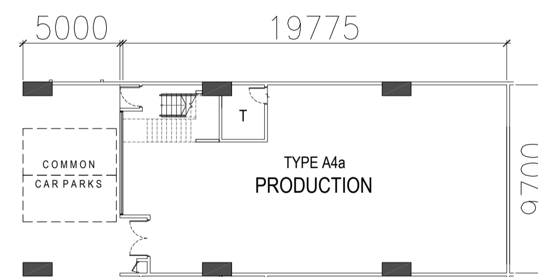
TYPE A4a - 1ST STOREY PLAN
