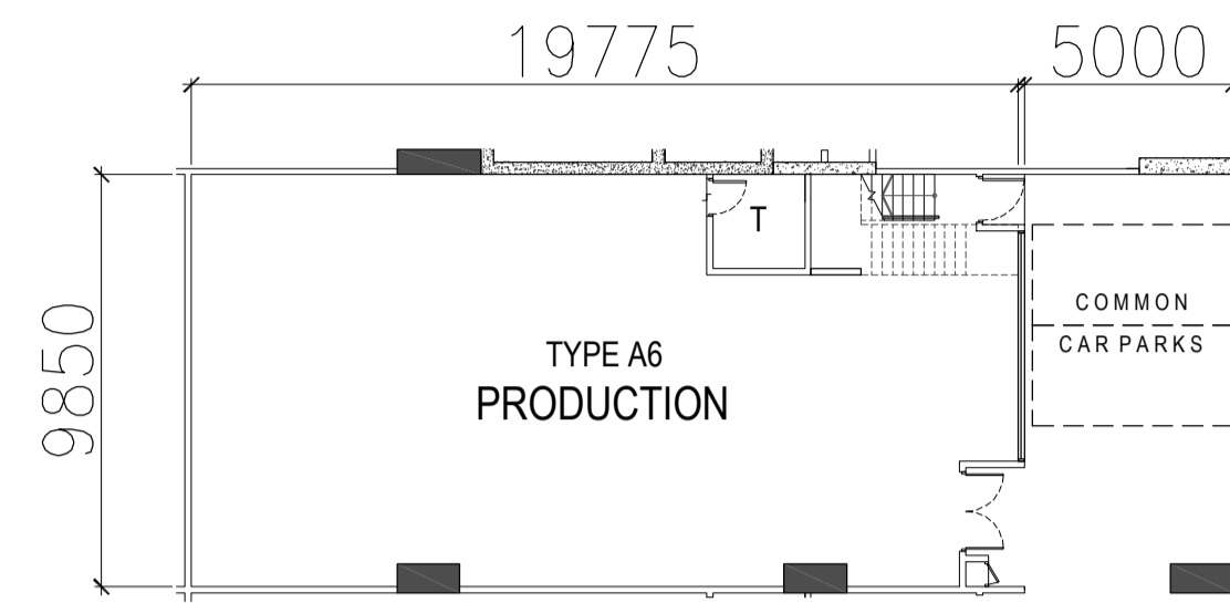
TYPE A6 - 1ST STOREY PLAN
