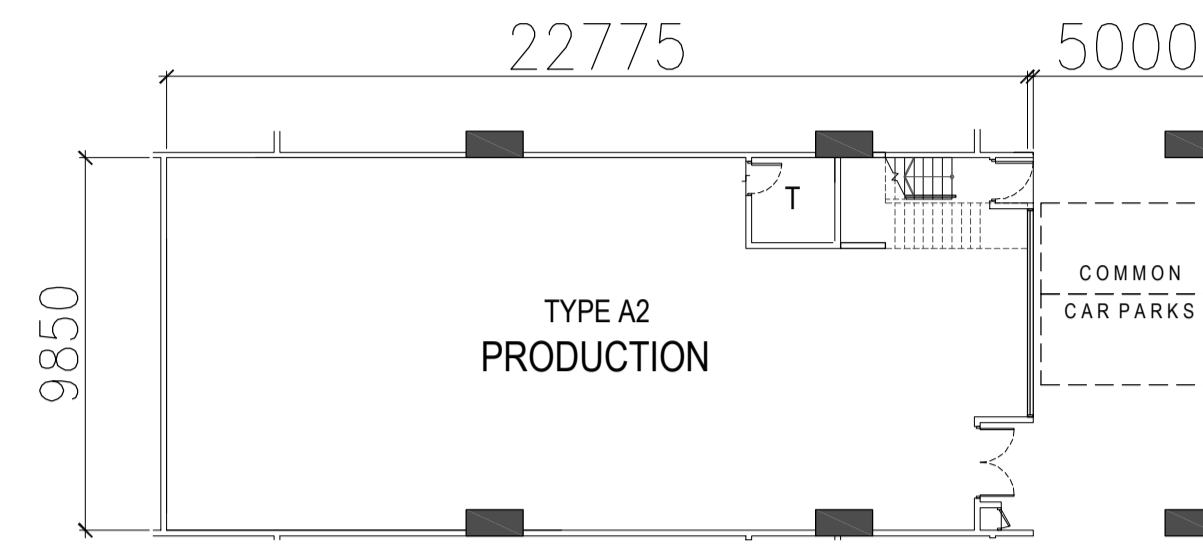
TYPE A2 - 1ST STOREY PLAN
