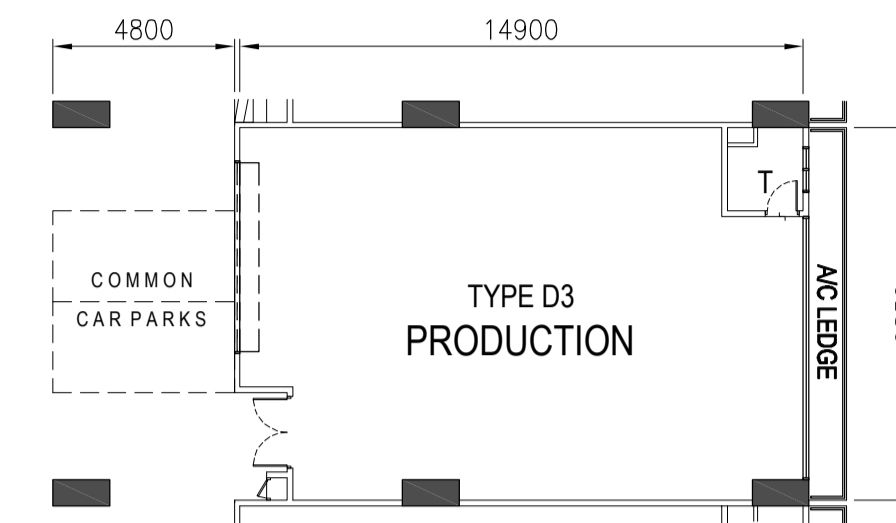
TYPE D3 - 9TH STOREY PLAN
