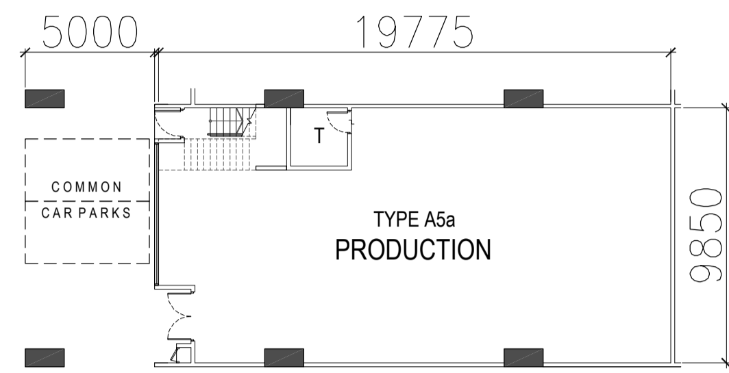
TYPE A5a - 1ST STOREY PLAN
