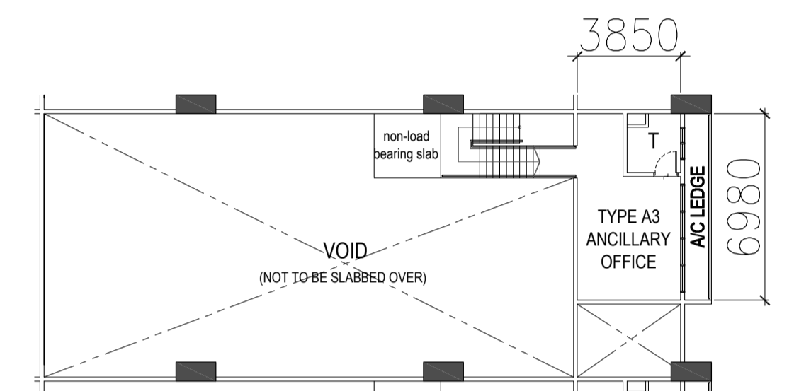
TYPE A3 - 1ST STOREY PLAN
