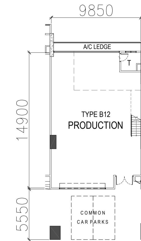
TYPE B12 - 2ND to 3RD STOREY PLAN
