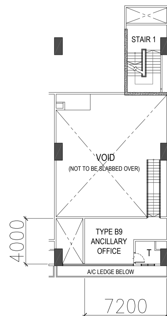
TYPE B9 - 2ND to 3RD MEZZ STOREY PLAN
