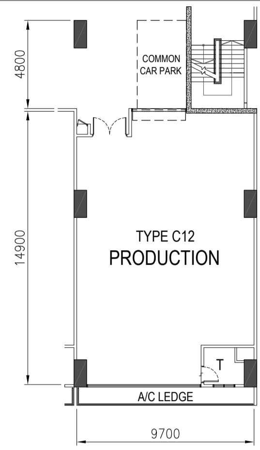
TYPE C12 - 5TH to 8TH STOREY PLAN
