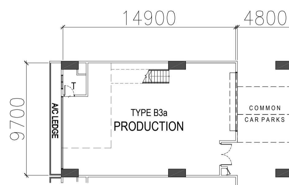
TYPE B3a - 2ND to 3RD STOREY PLAN
