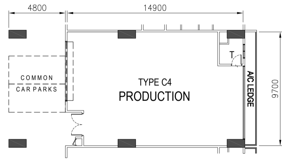
TYPE C4 - 5TH to 8TH STOREY PLAN
