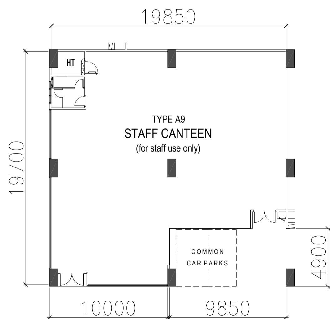
TYPE A9 - 1ST STOREY PLAN
