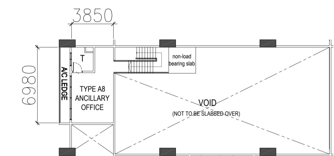
TYPE A8 - 1ST STOREY PLAN
