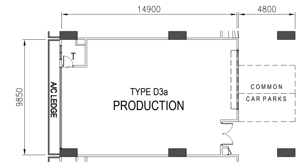
TYPE D3a - 9TH STOREY PLAN
