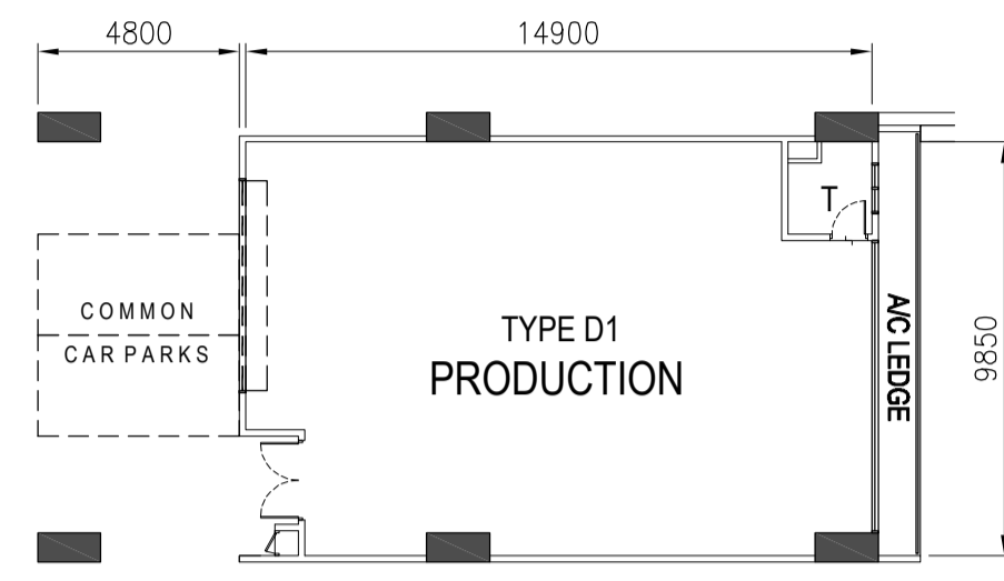
TYPE D1 - 9TH STOREY PLAN
