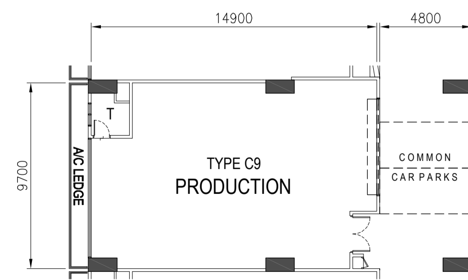
TYPE C9 - 5TH to 8TH STOREY PLAN
