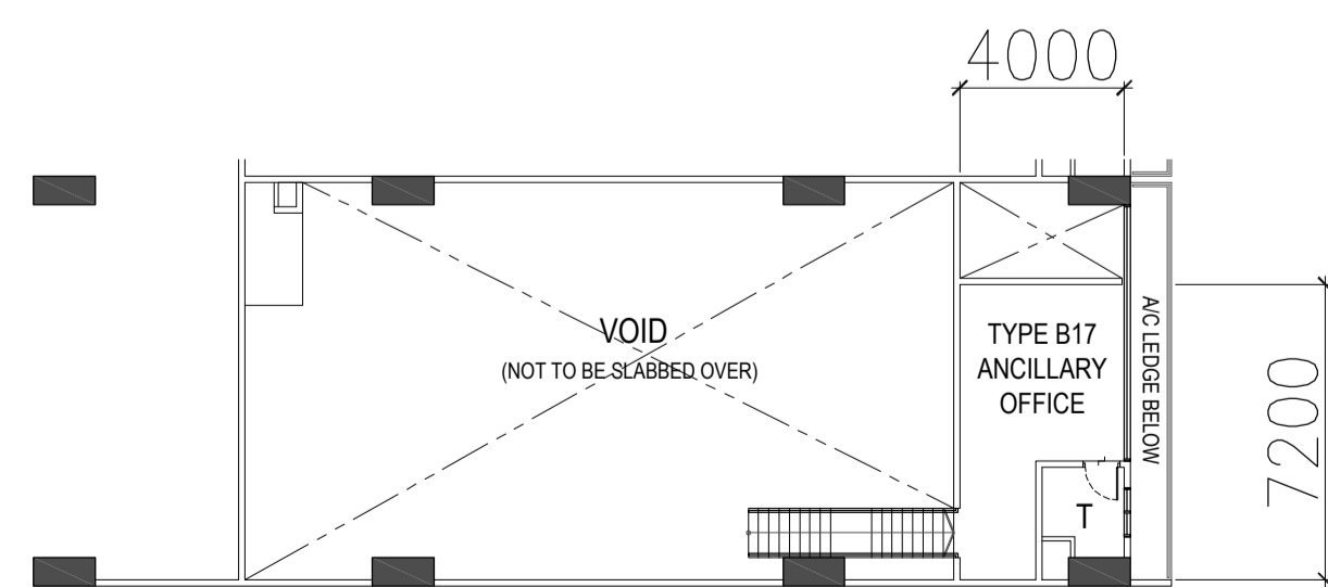
TYPE B17- 2ND to 3RD STOREY PLAN
