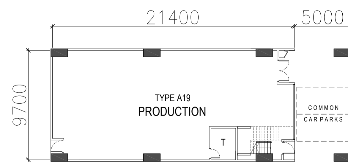
TYPE A19 - 1ST STOREY PLAN
