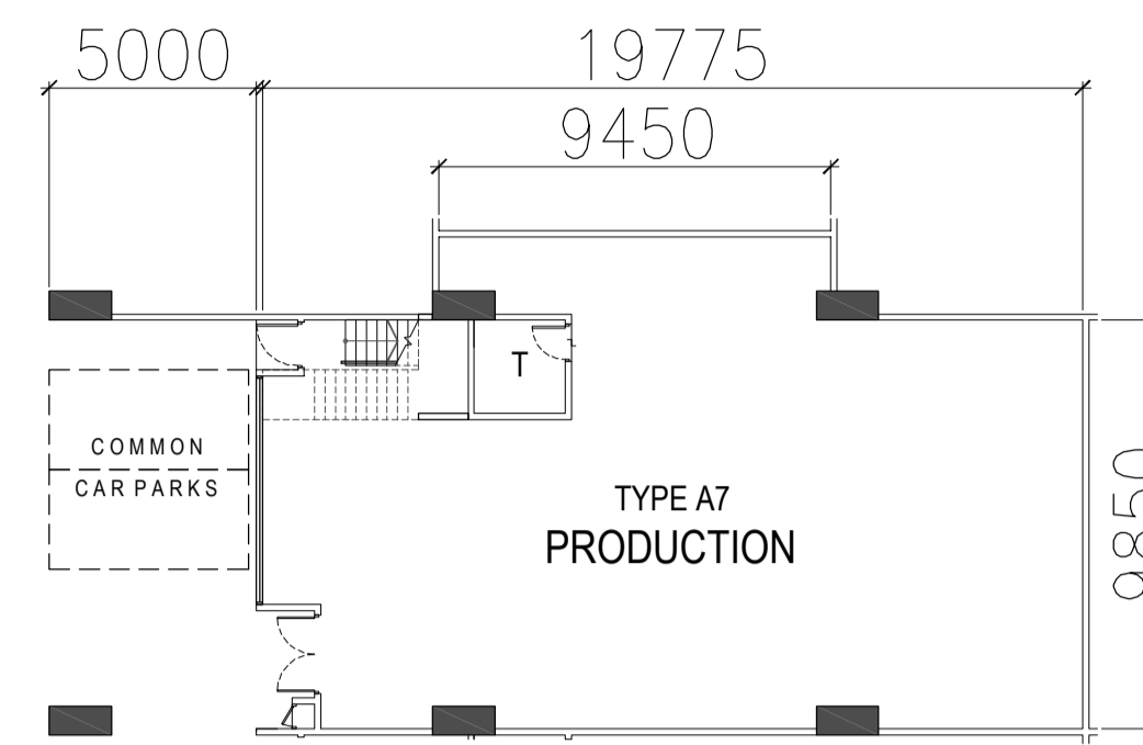
TYPE A7 - 1ST STOREY PLAN
