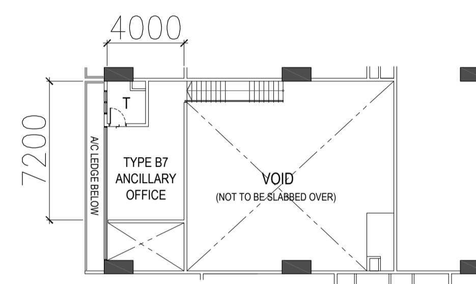
TYPE B7 - 2ND to 3RD STOREY PLAN
