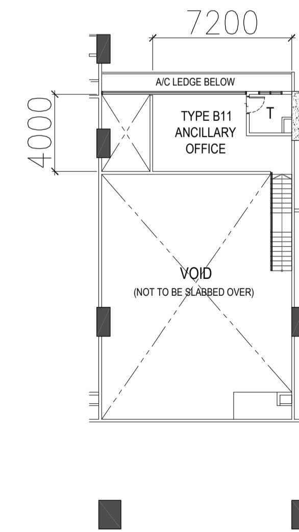
TYPE B11 - 2ND to 3RD MEZZ STOREY PLAN
