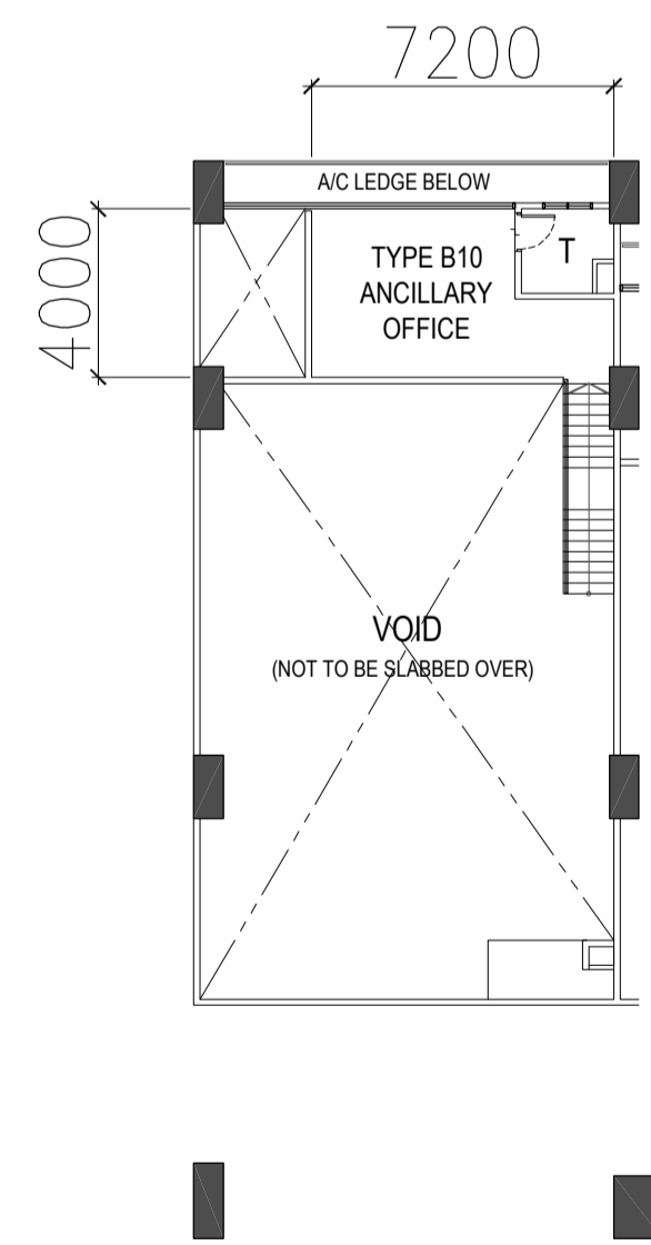
TYPE B10 - 2ND to 3RD MEZZ STOREY PLAN
