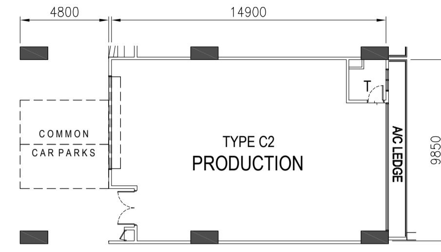
TYPE C2 - 5TH to 8TH STOREY PLAN
