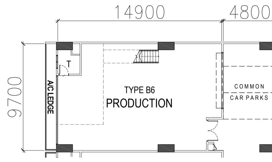
TYPE B6 - 2ND to 3RD STOREY PLAN
