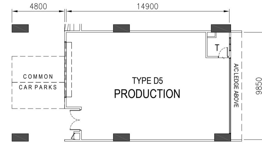
TYPE D5 - 9TH STOREY PLAN
