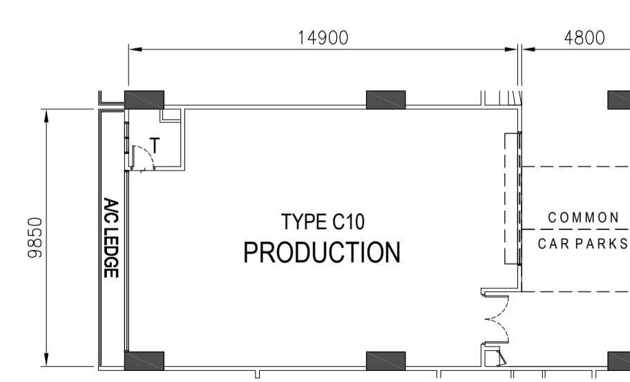
TYPE C10 - 5TH to 8TH STOREY PLAN
