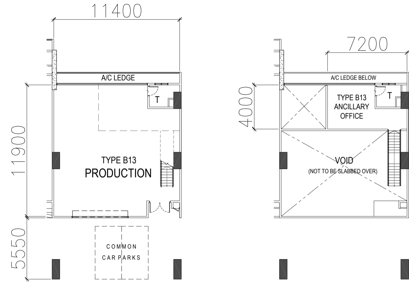
TYPE B13 - 2ND to 3RD STOREY PLAN TYPE B13 - 2ND to 3RD MEZZ STOREY PLAN
