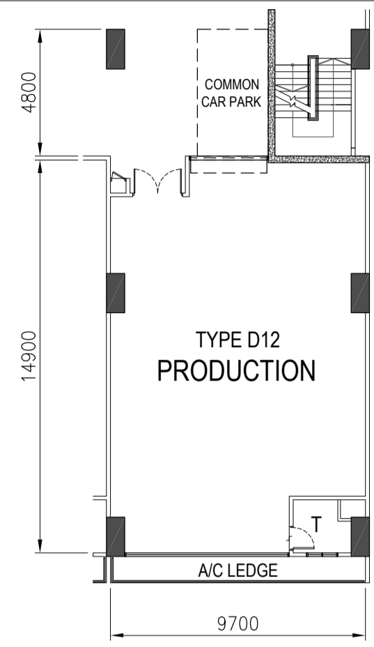
TYPE D12 - 9TH STOREY PLAN
