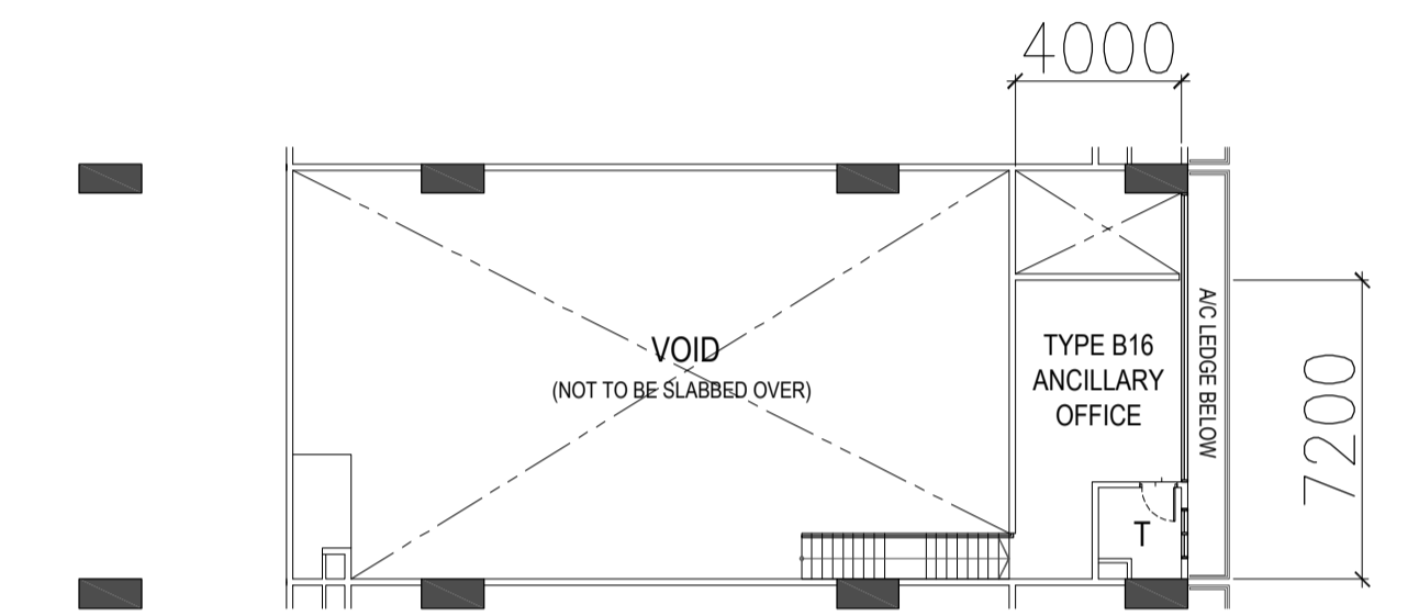
TYPE B16- 2ND to 3RD STOREY PLAN
