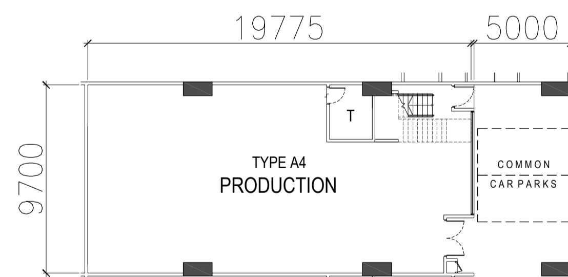
TYPE A4 - 1ST STOREY PLAN
