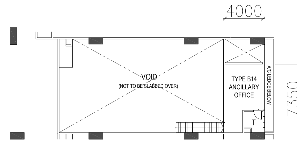
TYPE B14- 2ND to 3RD STOREY PLAN
