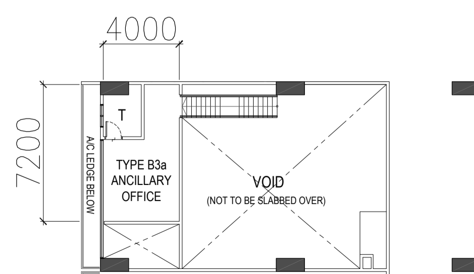
TYPE B3a - 2ND to 3RD STOREY PLAN
