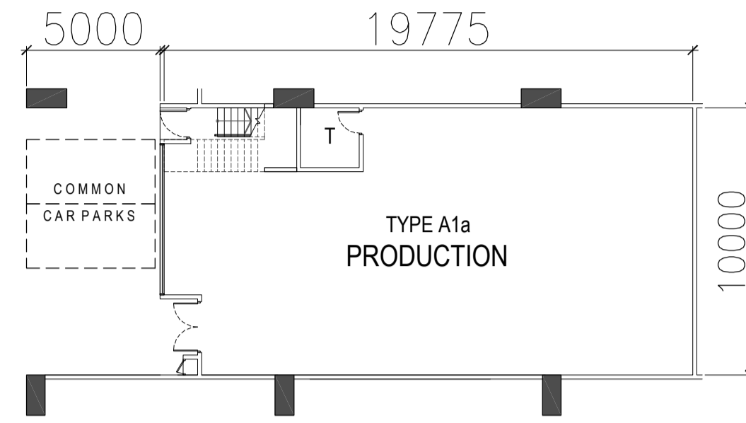
TYPE A1a - 1ST STOREY PLAN
