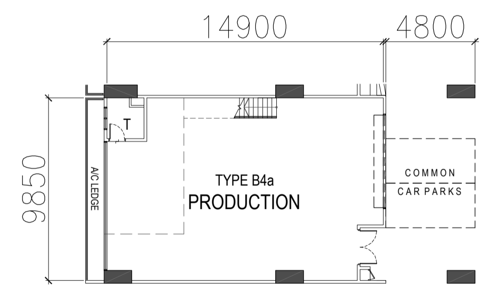
TYPE B4a - 2ND to 3RD STOREY PLAN
