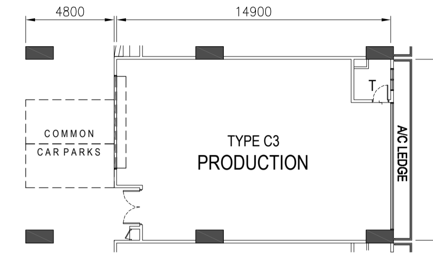
TYPE C3 - 5TH to 8TH STOREY PLAN
