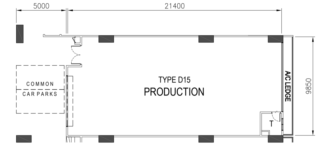
TYPE D15 - 9TH STOREY PLAN
