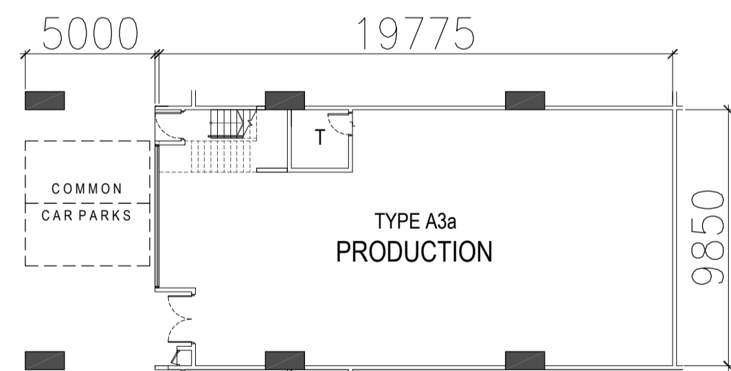
TYPE A3a - 1ST STOREY PLAN
