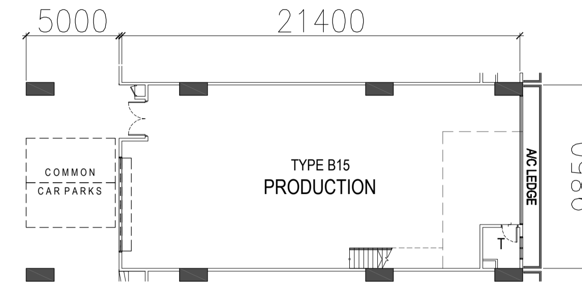
TYPE B15- 2ND to 3RD STOREY PLAN
