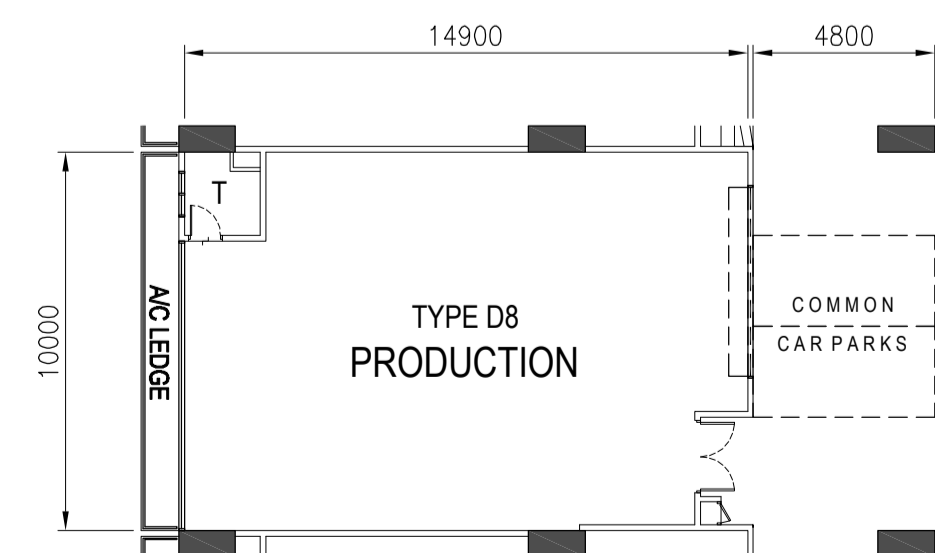
TYPE D8 - 9TH STOREY PLAN
