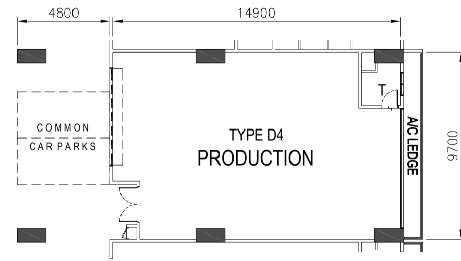
TYPE D4 - 9TH STOREY PLAN
