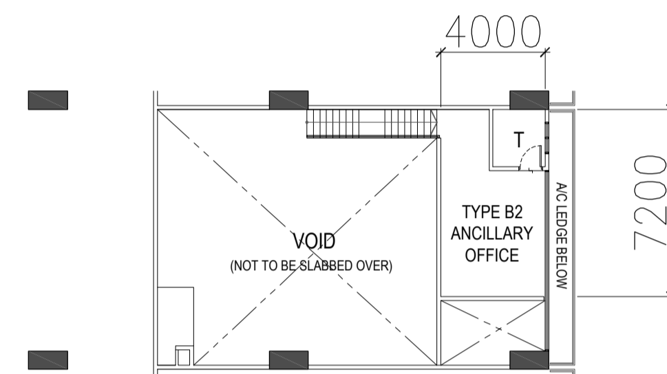
TYPE B2- 2ND to 3RD STOREY PLAN
