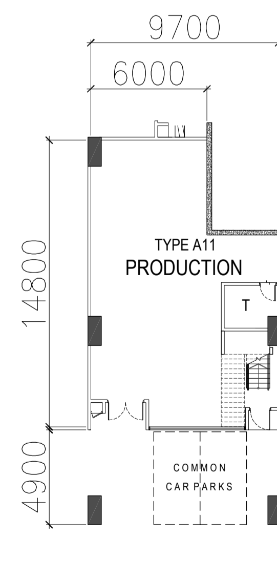
TYPE A11 - 1ST STOREY PLAN
