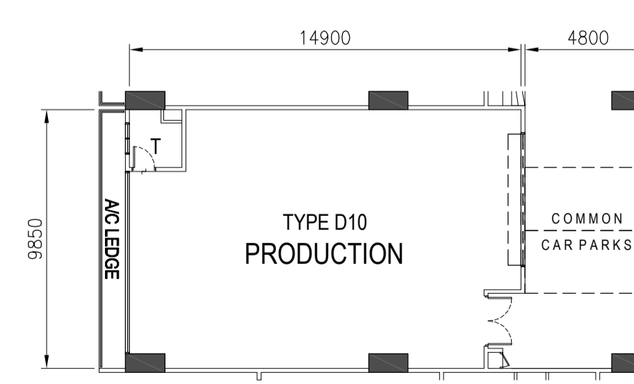
TYPE D10 - 9TH STOREY PLAN
