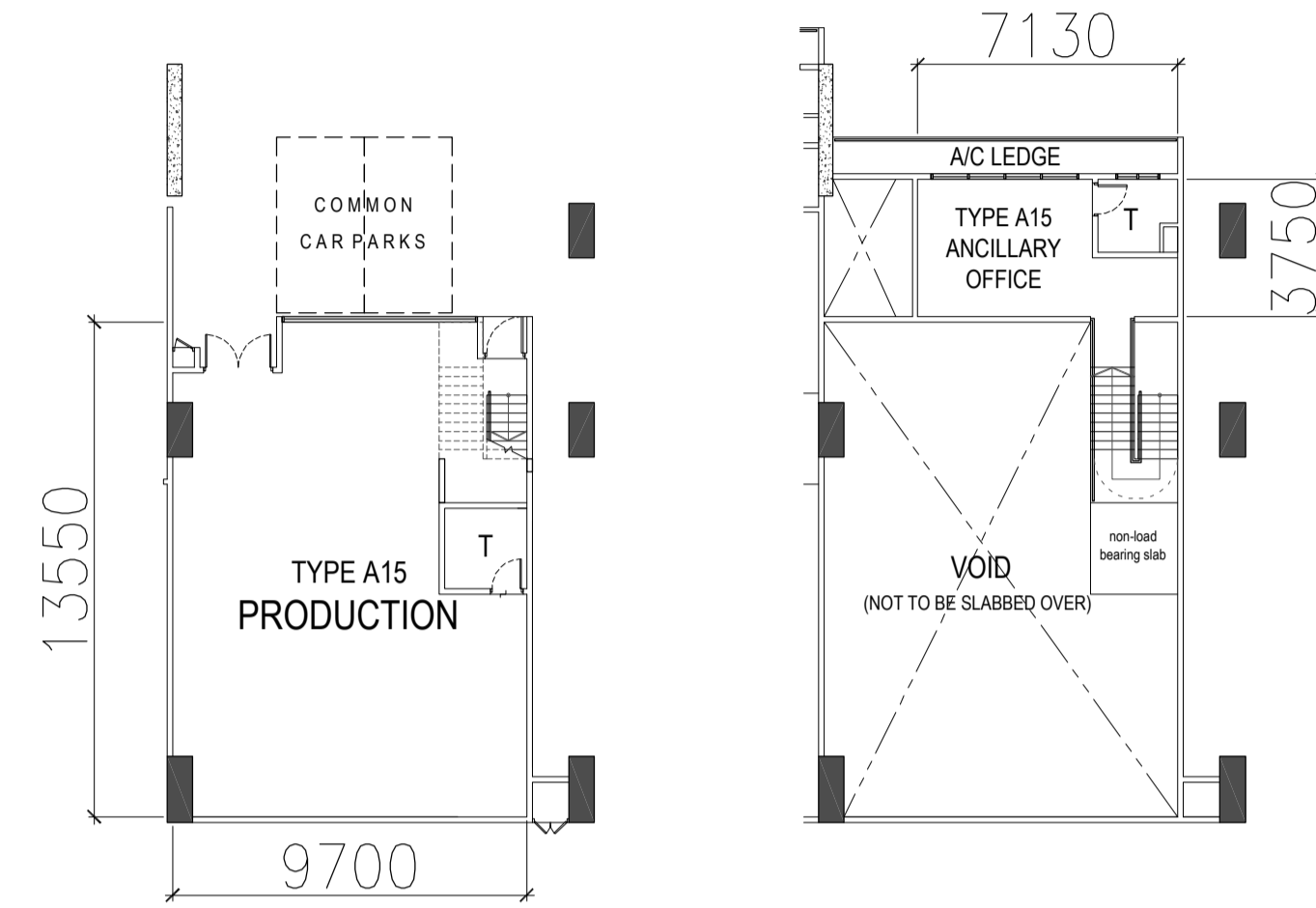
TYPE A15 - 1ST STOREY PLAN
