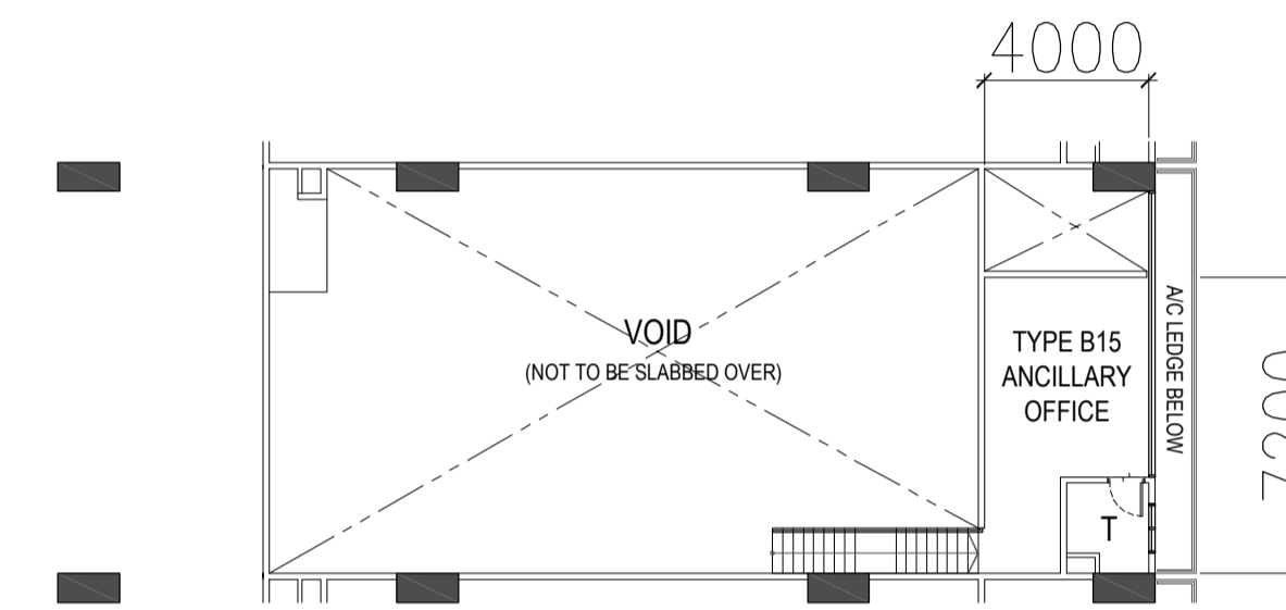
TYPE B15- 2ND to 3RD STOREY PLAN
