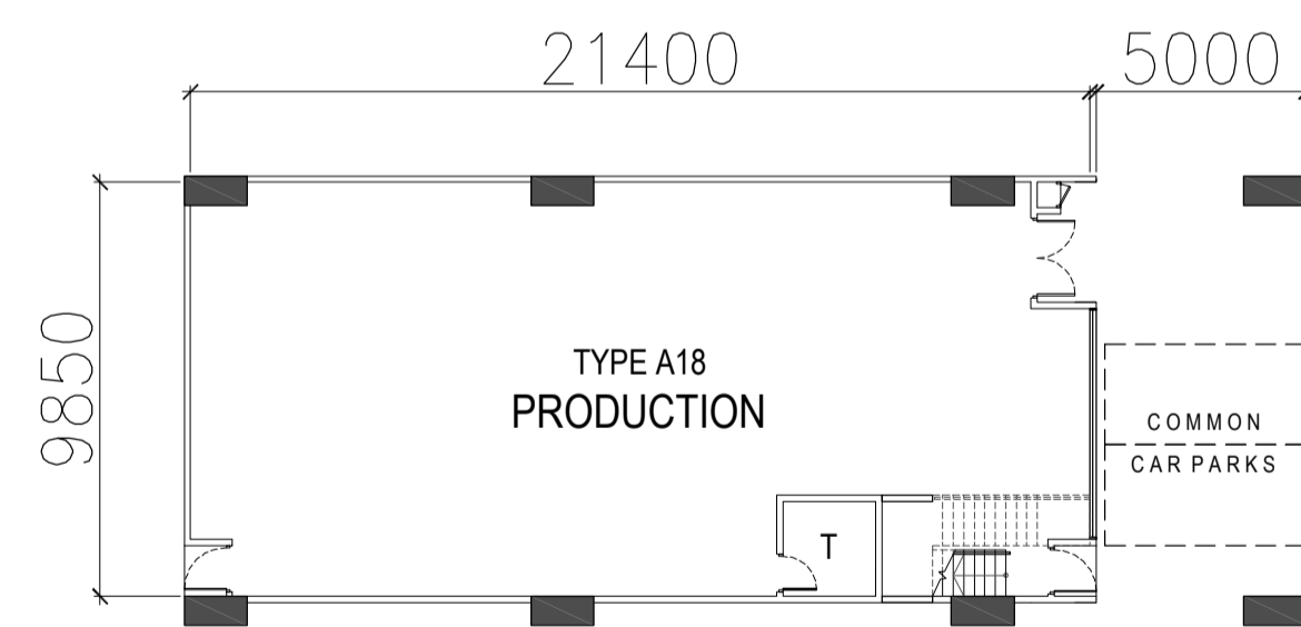
TYPE A18 - 1ST STOREY PLAN
