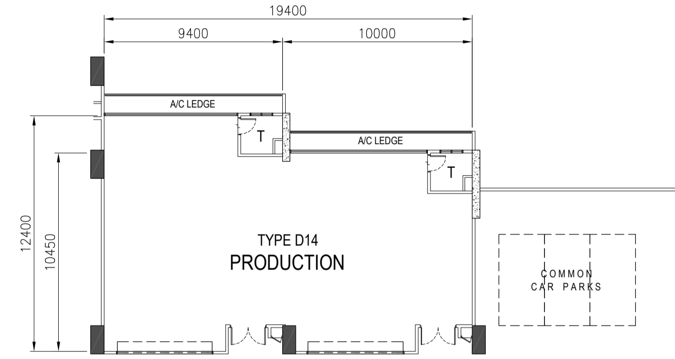
TYPE D14 - 9TH STOREY PLAN
