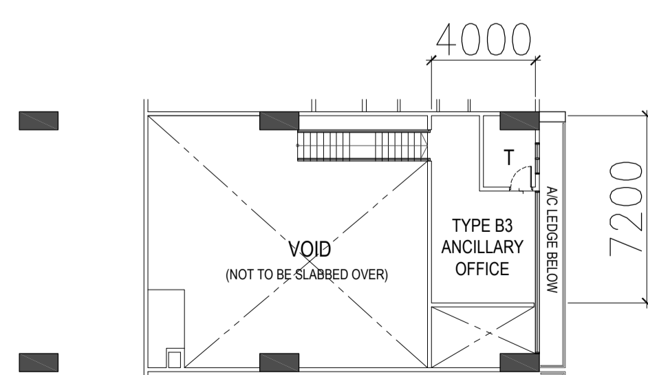
TYPE B3- 2ND to 3RD STOREY PLAN
