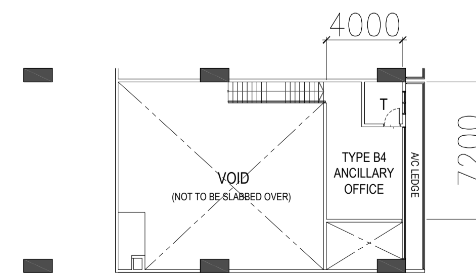
TYPE B4 - 2ND to 3RD STOREY PLAN
