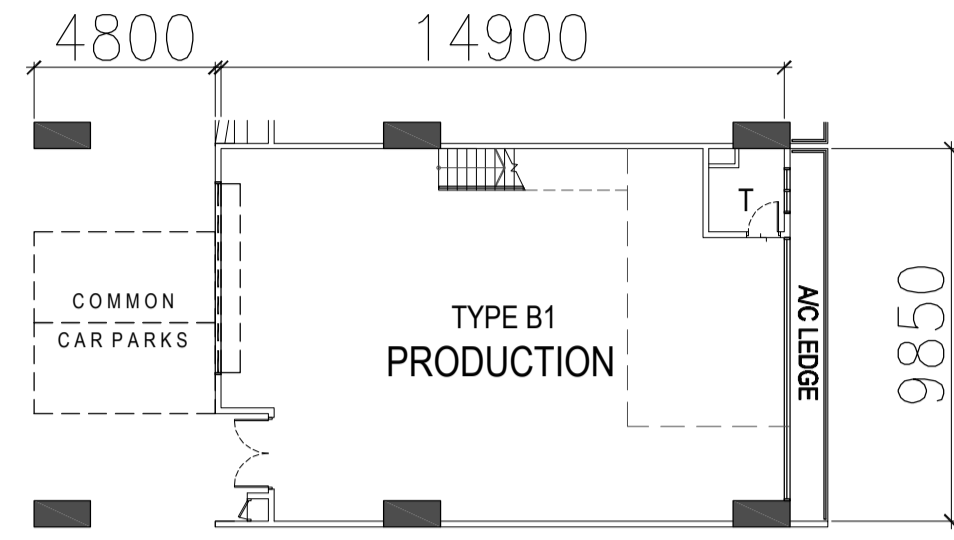
TYPE B1 - 2ND to 3RD STOREY PLAN
