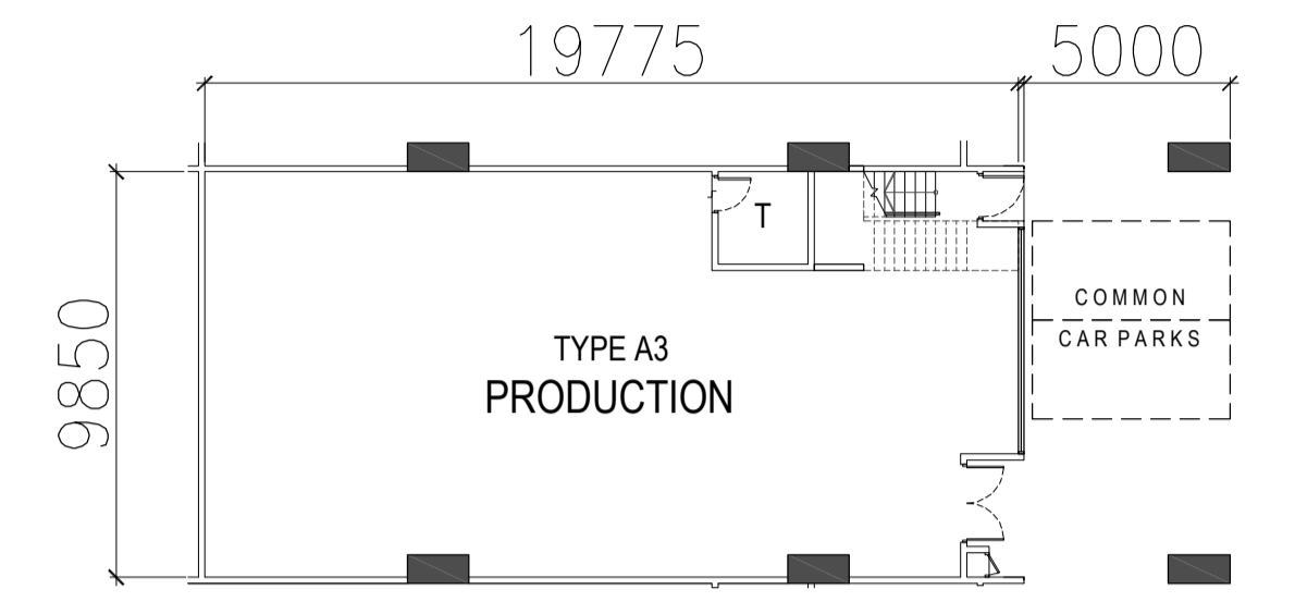
TYPE A3 - 1ST STOREY PLAN
