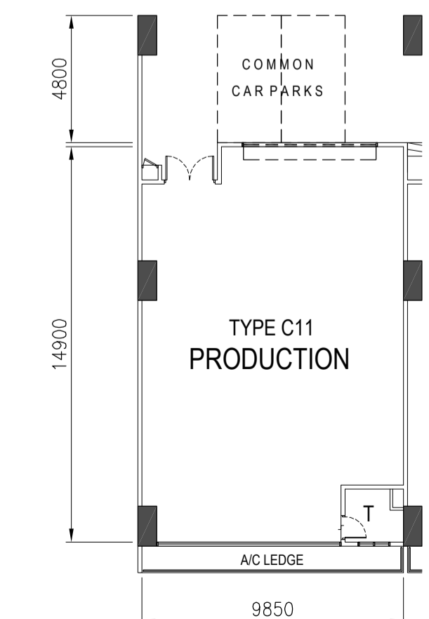
TYPE C11 - 5TH to 8TH STOREY PLAN
