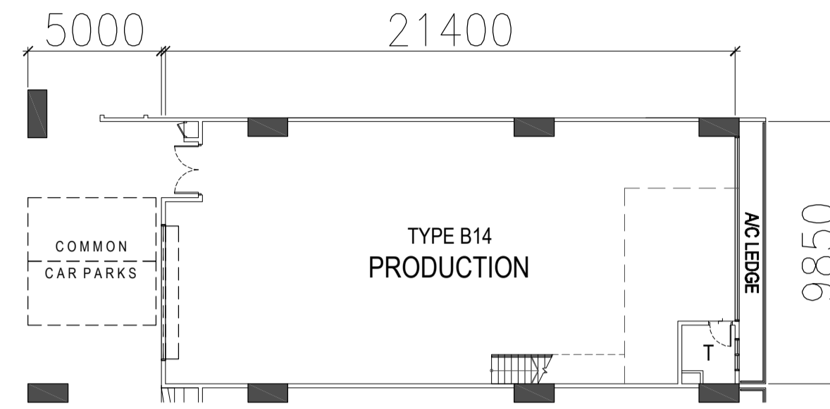
TYPE B14- 2ND to 3RD STOREY PLAN
