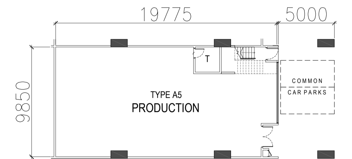
TYPE A5 - 1ST STOREY PLAN
