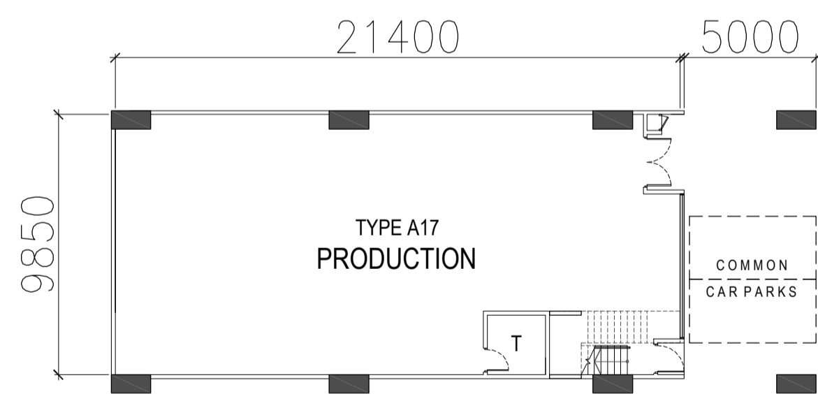
TYPE A17 - 1ST STOREY PLAN
