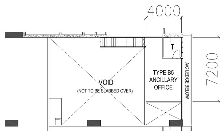
TYPE B5 - 2ND to 3RD STOREY PLAN
