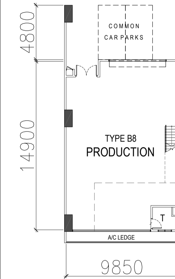
TYPE B8 - 2ND to 3RD STOREY PLAN
