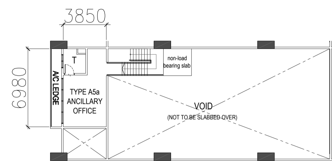
TYPE A5a - 1ST STOREY PLAN
