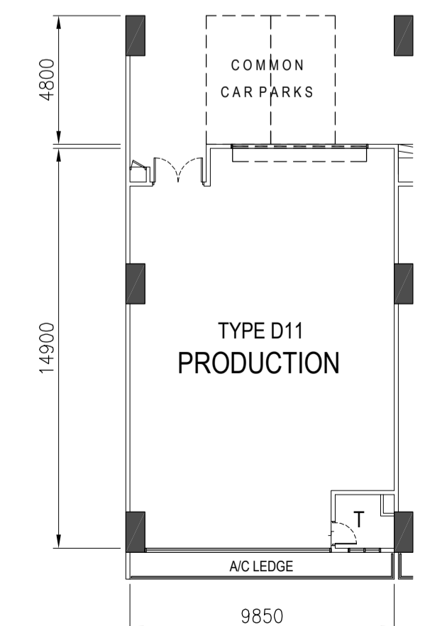
TYPE D11 - 9TH STOREY PLAN
