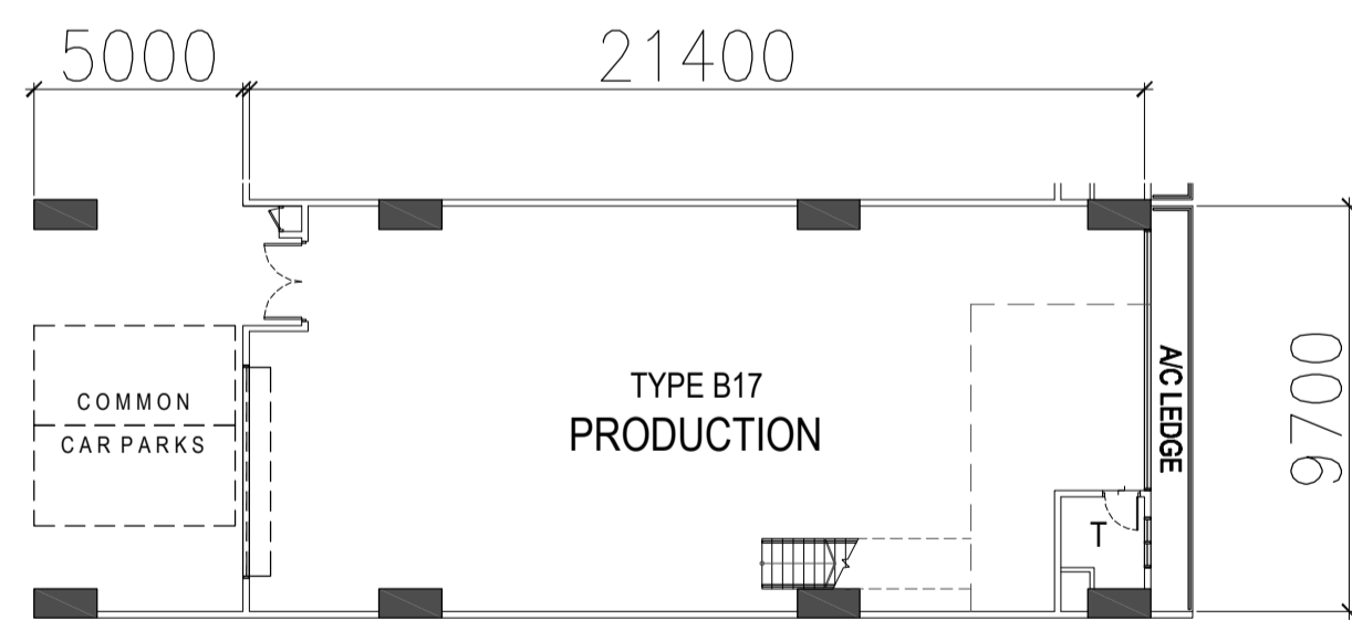
TYPE B17- 2ND to 3RD STOREY PLAN
