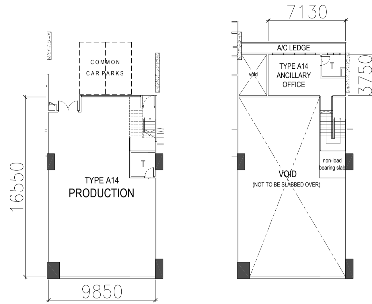
TYPE A14 - 1ST STOREY PLAN
