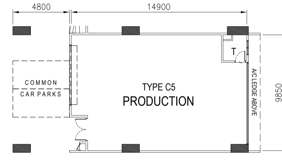
TYPE C5 - 5TH to 8TH STOREY PLAN
