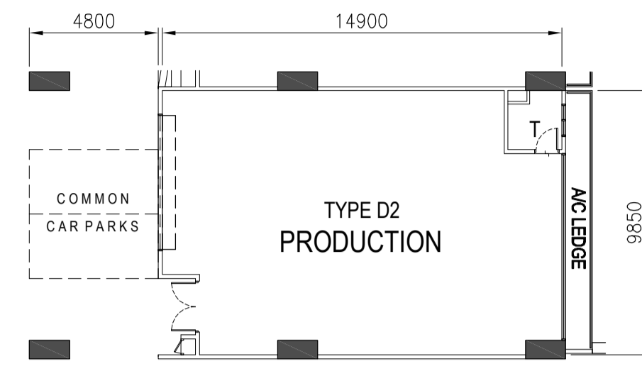
TYPE D2 - 9TH STOREY PLAN
