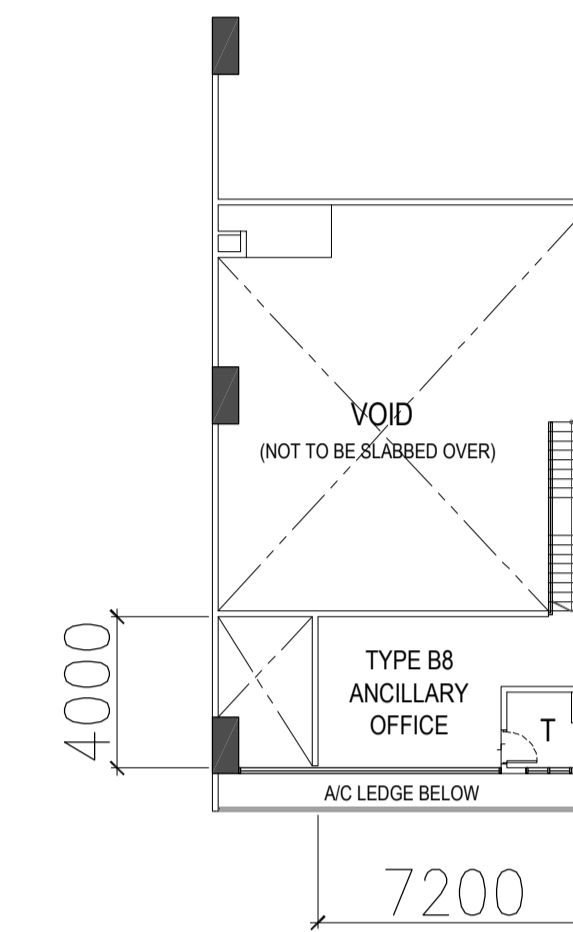
TYPE B8 - 2ND to 3RD MEZZ STOREY PLAN
