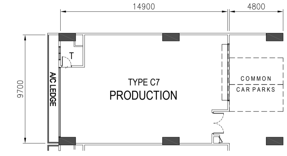
TYPE C7 - 5TH to 8TH STOREY PLAN
