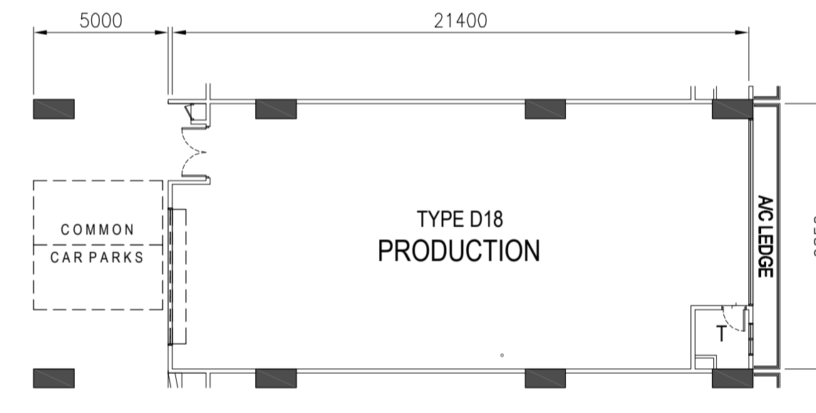
TYPE D18 - 9TH STOREY PLAN
