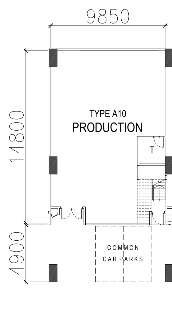
TYPE A10 - 1ST STOREY PLAN
