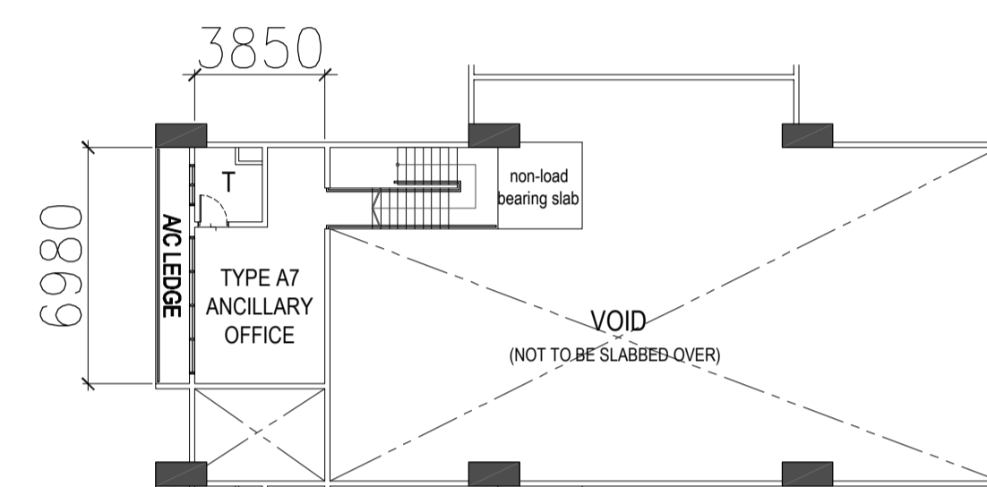
TYPE A7 - 1ST STOREY PLAN
