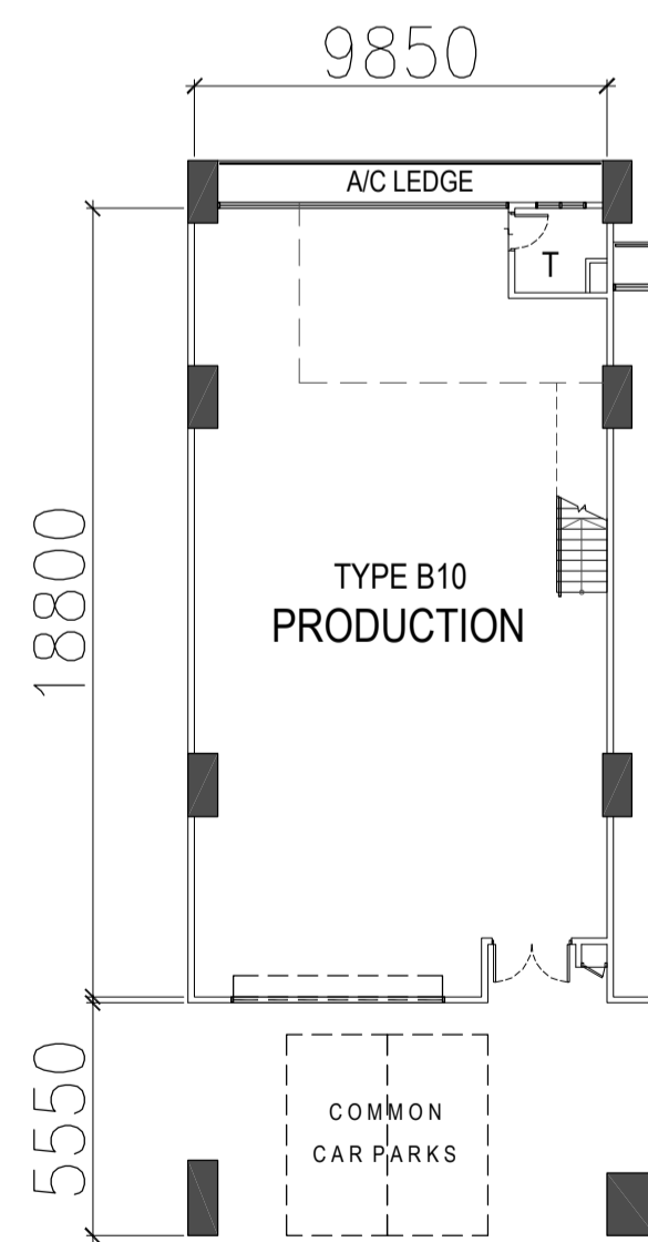
TYPE B10 - 2ND to 3RD STOREY PLAN
